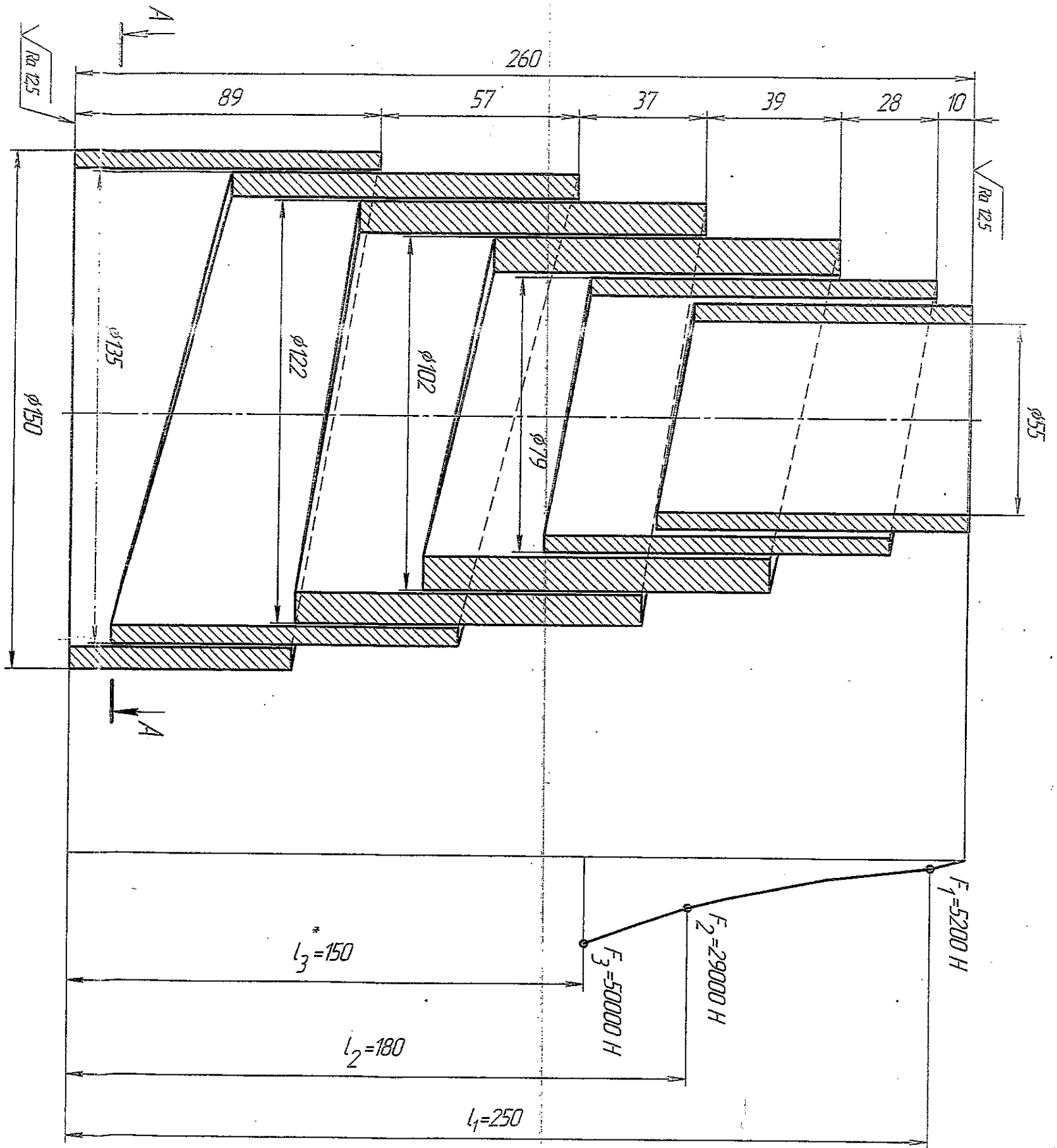
Q, (1:2)
